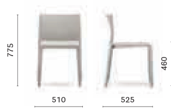
670 Polypropylene side chair
