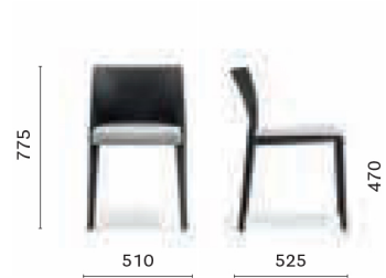
671/2 Polypropylene side chair, upholstered seat
