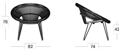
Cruz lazy chair
